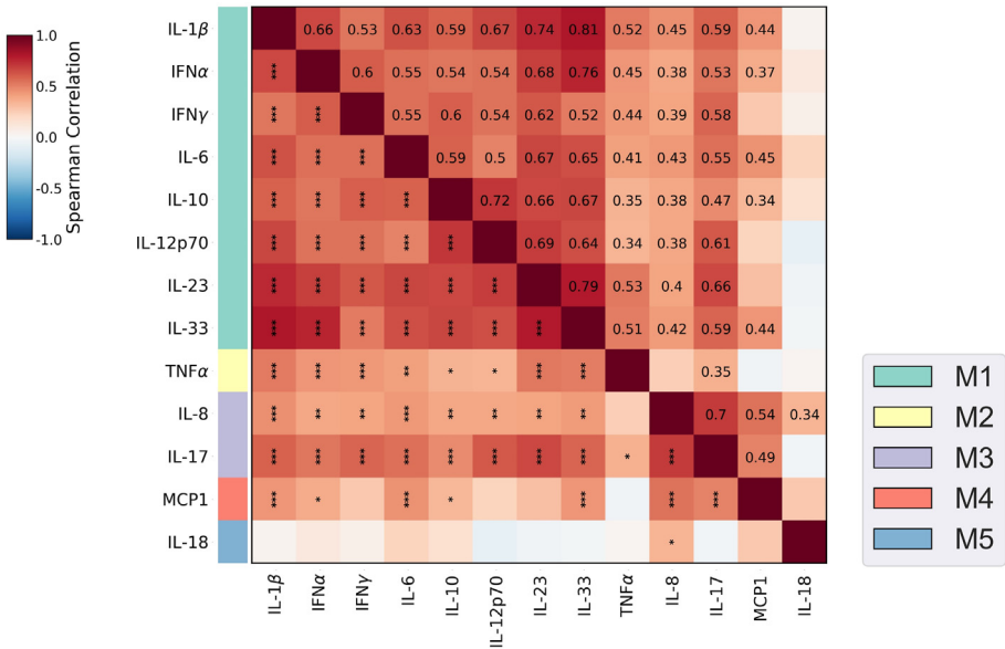
Fig. 2. Cytokine interactions modules among CD patients at baseline. A heatmap portraying Spearman correlations and their p-values corrected using family-wise error rate (FWER) for multiple hypothesis adjustment (Methods). Numbers indicate the correlations and asterisks indicate the FWER-adjusted p-values of these correlations: *p < 0.05, **p < 0.005 and *** for p < 0.0005. The colored stripes represent the assignment of cytokines to modules (M1-M5) by their correlations using the CytoMod algorithm (Cohen et al., 2019).
